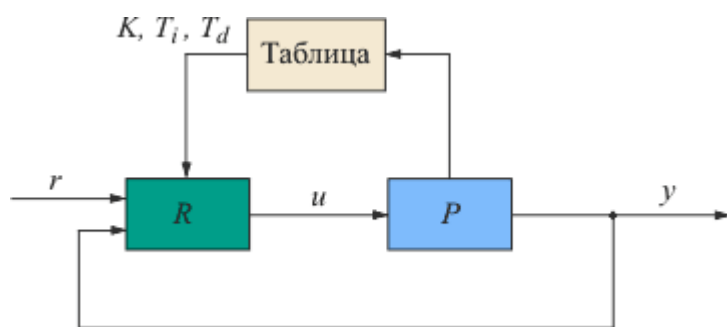
Fig. 1. Adaptive control using parameters previously recorded in the table
