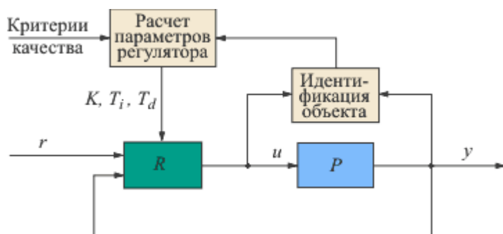
Fig. 2. The overall structure of the system with automatic configuration
